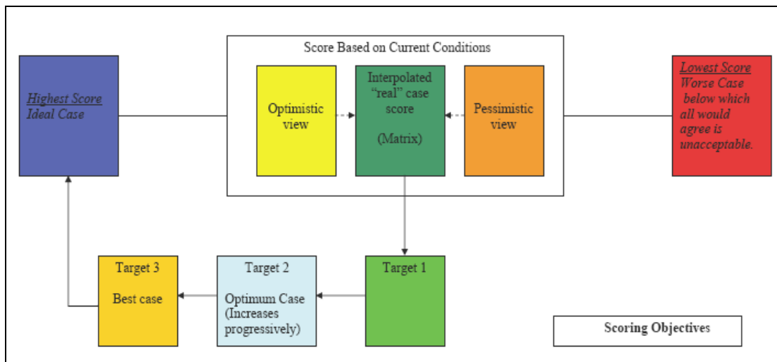
Figure 2.7 Conceptual scoring
